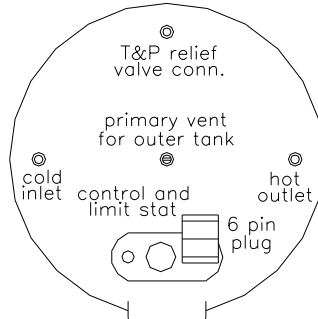
VIEW OF TANK TOP
