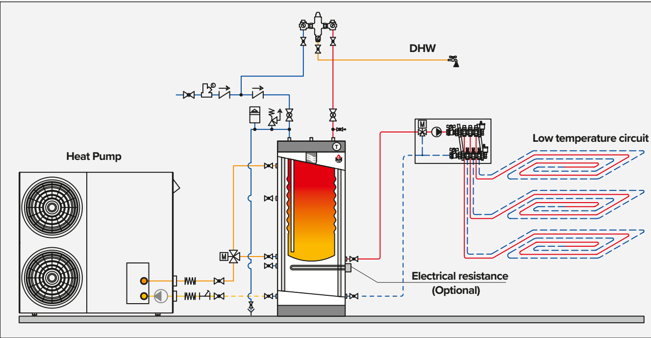
Scheme 1 - Unvented system showing a variable temperature circuit with heat pump and underfloor heating.
