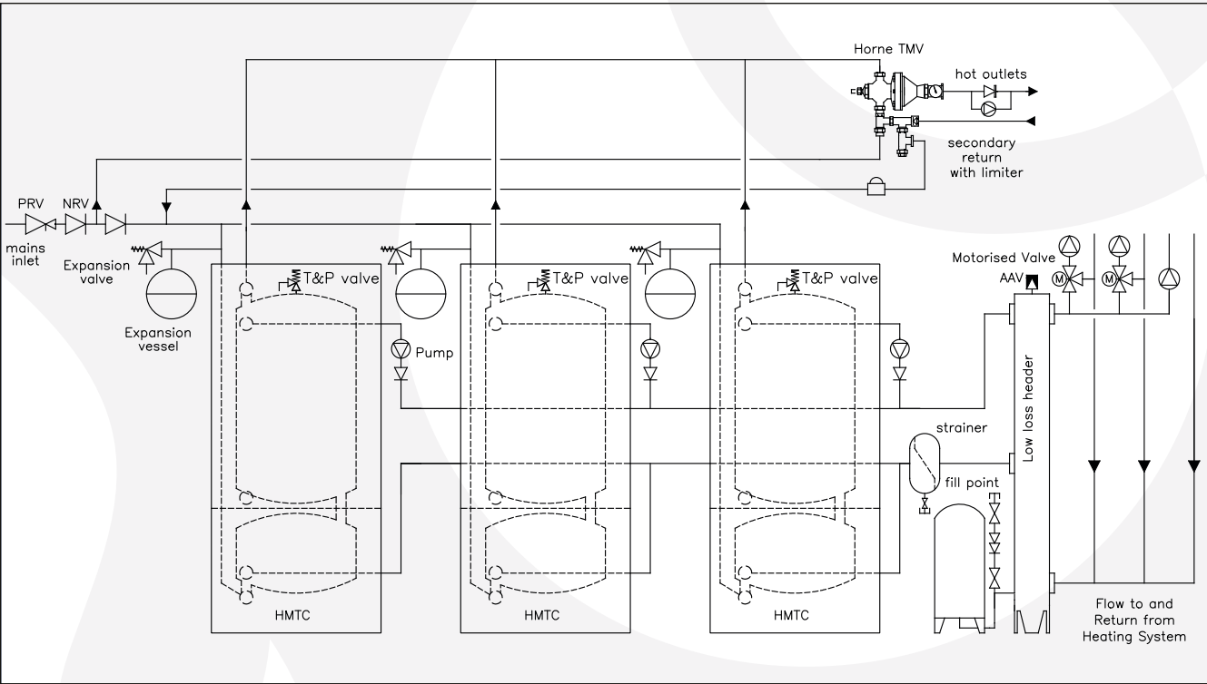
Scheme 3 - HeatMaster® hydraulic cascade with low loss header providing domestic hot water and space heating.
