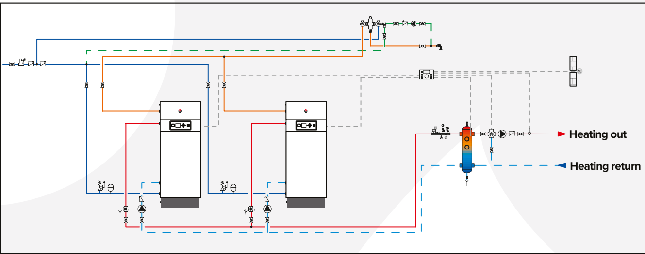
Scheme 4 - HeatMaster® cascade system with control wiring.
