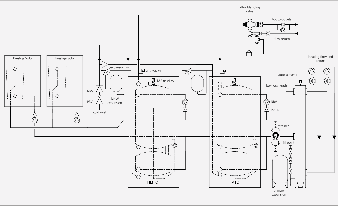
Scheme 2 - HeatMaster® and Prestige® full cascade incorporating Prestige® boilers for additional kilowatt input. The only total condensing heating and hot water installation.
