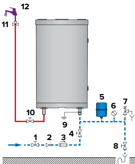
Installation verticale
