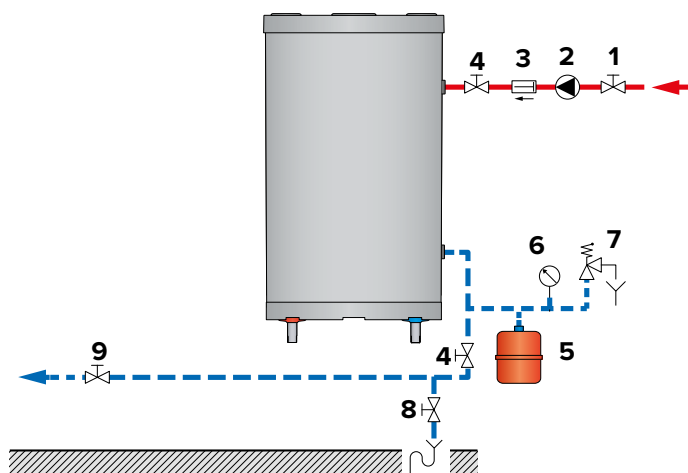
Vertikale Installation
