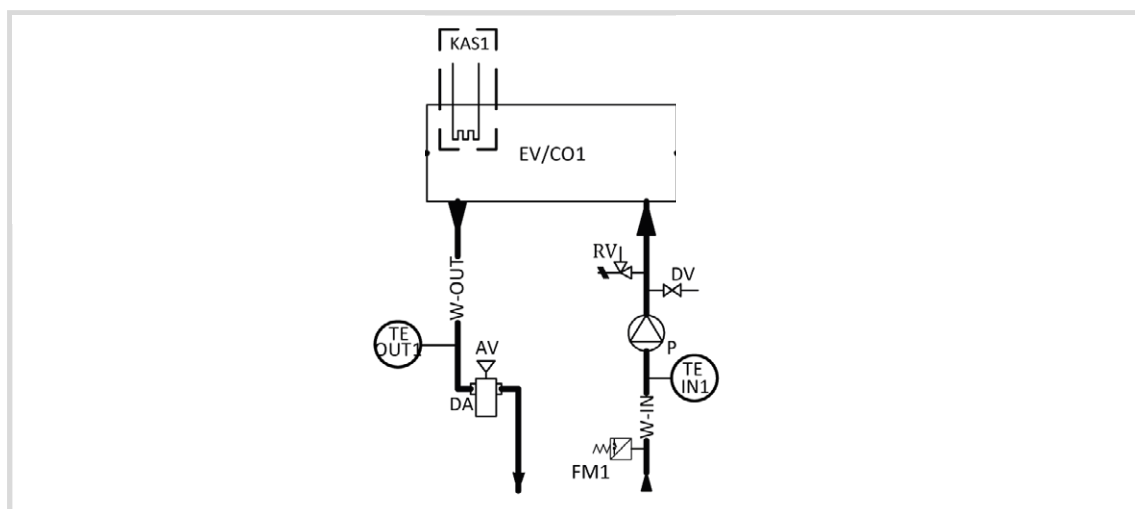
figure 11 - Circuit hydraulique
