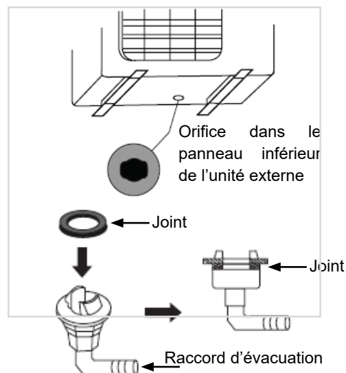
figure 9 - Evacuations des condensats
